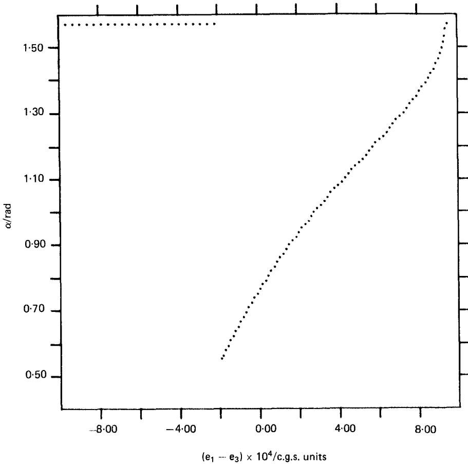
Figure 5. Variation of \alpha with e_1 - e_3 calculated for \Delta\epsilon = 0 and including the elastic anisotropy. Note that \alpha does not go to zero in this case.
