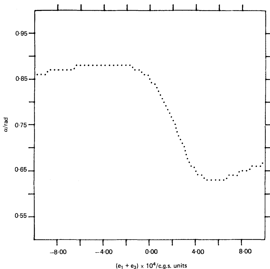
Figure 6. Variation of \alpha with e_1 + e_3 calculated for \Delta\varepsilon = 0 and including the elastic anisotropy. In this and some of the other figures the coarseness in the plot is due to a relatively low resolution on the monitor from which a hard copy was obtained.
