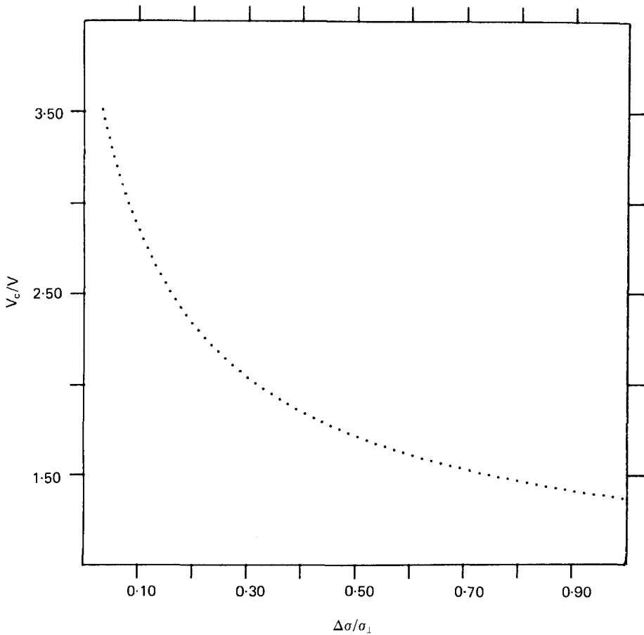
Figure 10. Variation of the critical voltage V_c with \Delta\sigma/\sigma_{\perp} .
