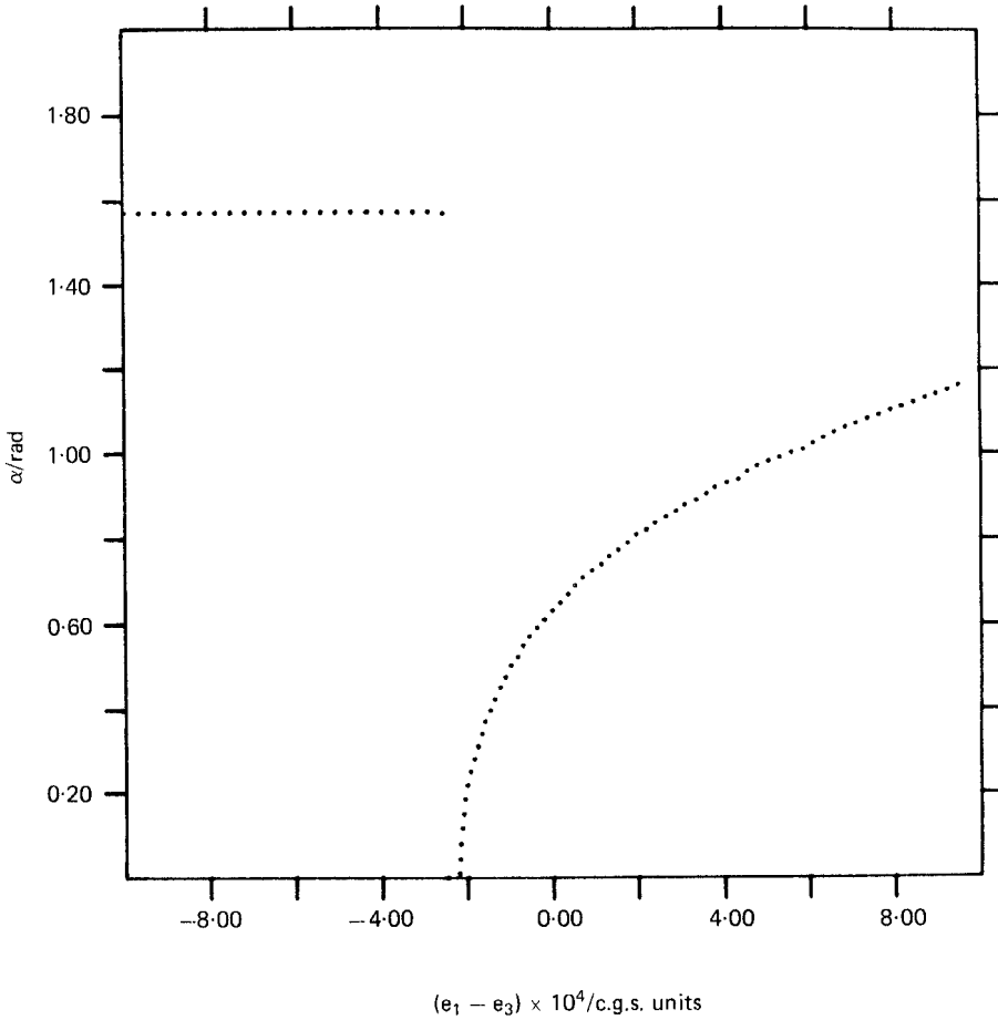
Figure 3. Variation of \alpha with e_1 - e_3 calculated for \Delta\varepsilon = 0 and K_3 = K_2 = K_1 . Note that \alpha = 0 for a very small range of negative values of e_1 - e_3 , and below this range the longitudinal flexoelectric domains are obtained.
