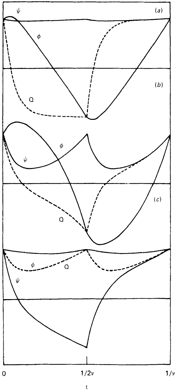
Figure 17. Variations of \psi , \phi and Q with time for one period of the applied square-wave electric field: (a) just above the threshold in the conduction regime at 40 Hz; (b) slightly below the restabilization curve at 100 Hz; (c) in the dielectric regime at 170 Hz. The values of the material parameters used in these calculations are the same as in figure 15.
