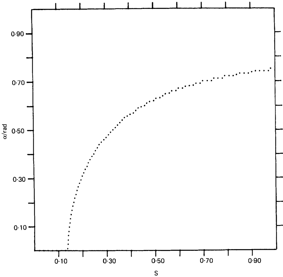
Figure 9. Variation of \alpha with the factor S by which the flexoelectric coefficients are decreased.
