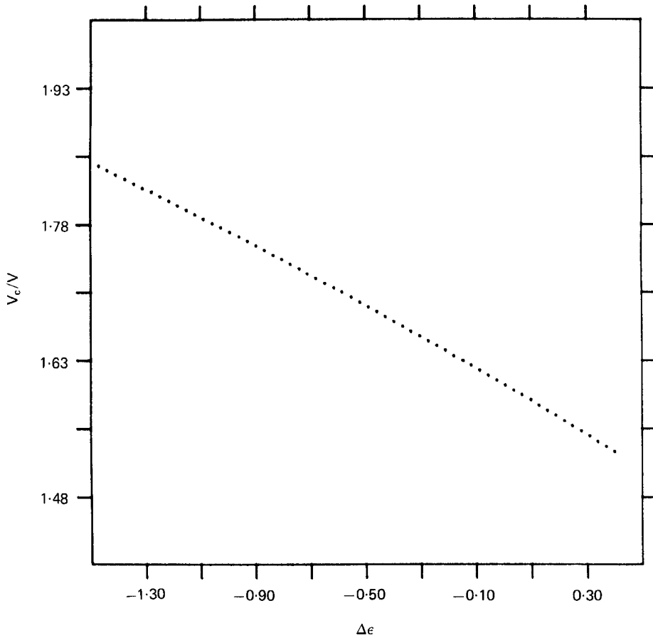
Figure 7. Variation of the critical voltage V_c with the dielectric anisotropy \Delta\epsilon .
