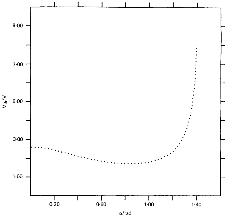
Figure 2. Variation of D.C. threshold voltage V_{th} with \alpha calculated for the standard values of the MBBA parameters listed in the table.
