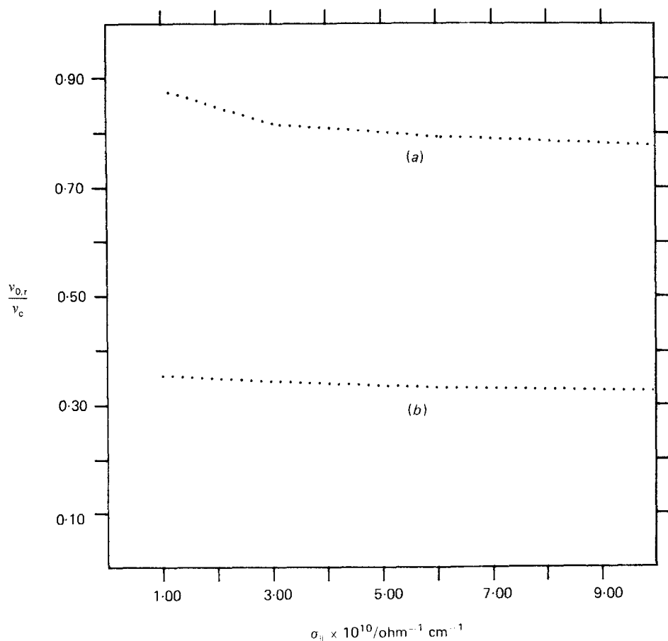
Figure 18. Variation of the ratios of frequencies v_0/v_c (curve (a)) and v_r/v_c (curve (b)) with \sigma_{||} .
