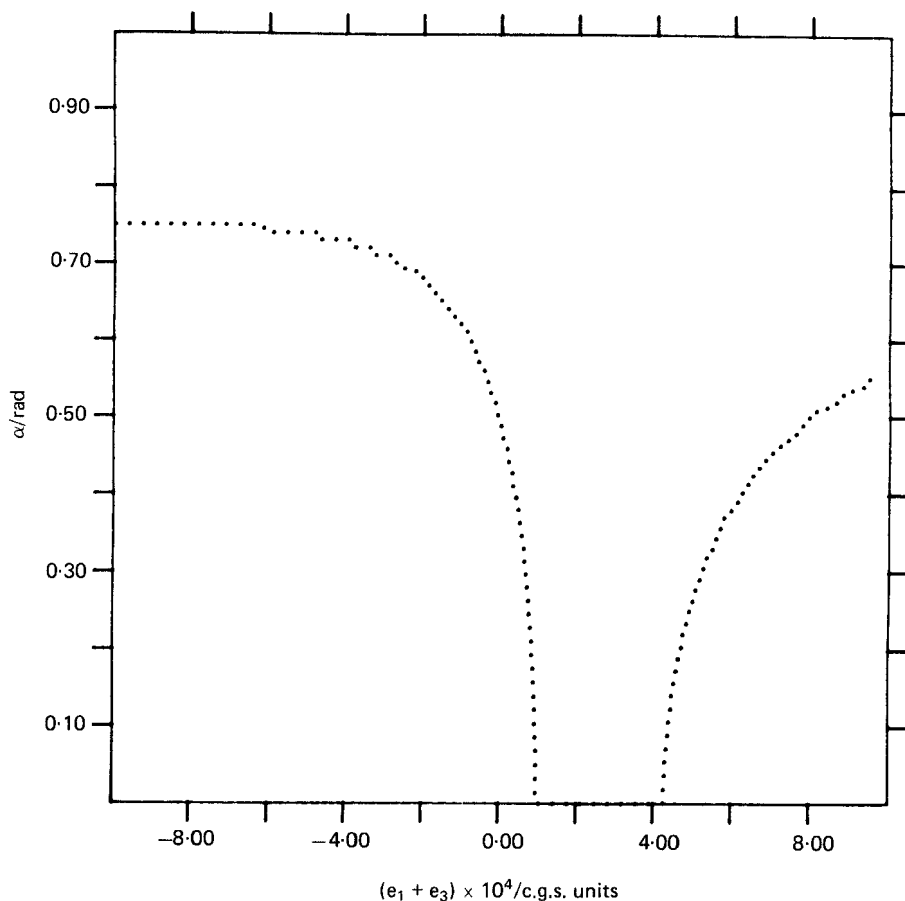
Figure 4. Variation of \alpha with e_1 + e_3 calculated for \Delta\varepsilon = 0 and K_3 = K_2 = K_1 . Note that \alpha = 0 for a small range of positive values of e_1 + e_3 .
