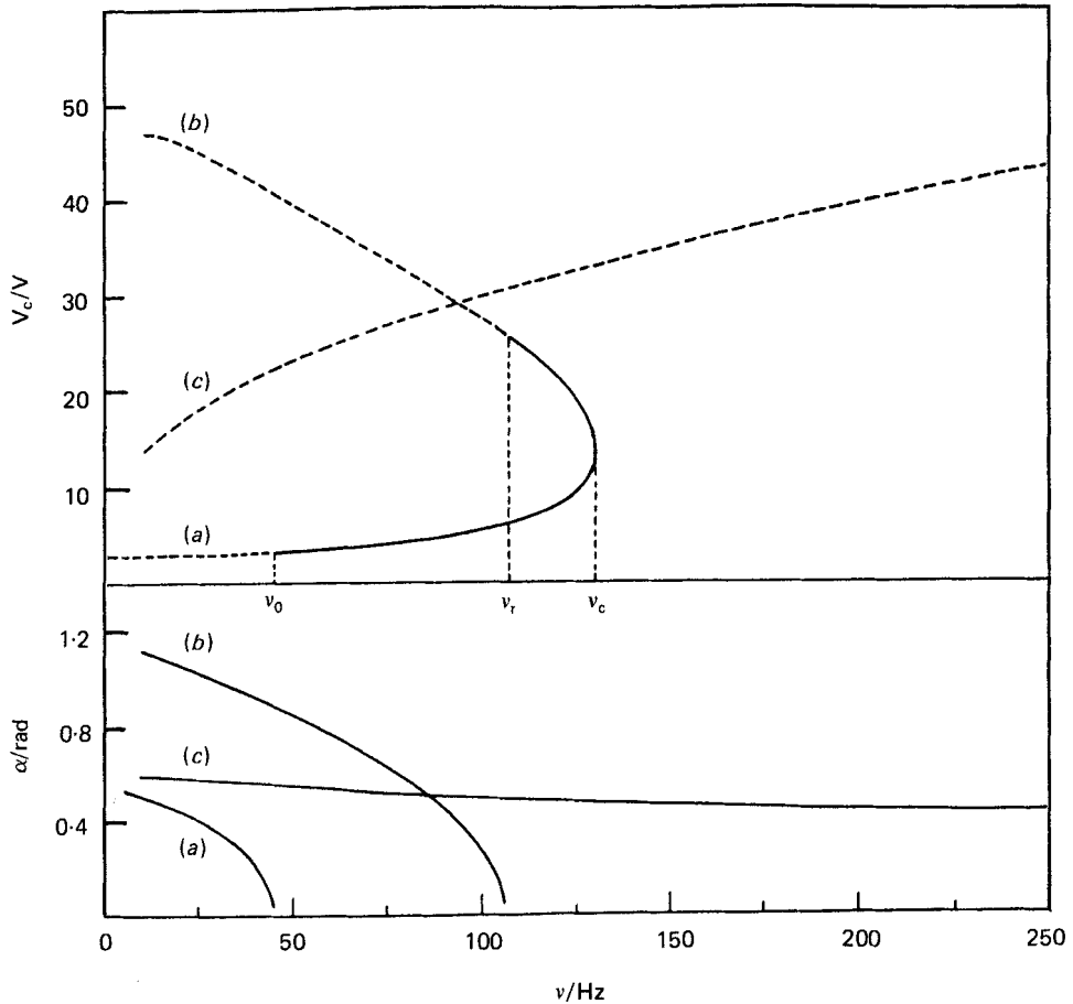
Figure 15. Upper section: Threshold voltage (curve (a)) and restabilization voltage (curve (b)) as functions of the frequency in the conduction regime for MBBA with \sigma_{\parallel} = 3 \times 10^{-10} \text{ ohm}^{-1} \text{ cm}^{-1} . The low-frequency portions indicated by dashed lines are characterized by non-zero values of \alpha . The frequency dependence of the voltage at threshold for a 20 \mu\text{m} thick sample in the dielectric regime is shown by curve (c). Lower section: Variations of tilt angle \alpha of the oblique rolls with frequency. (a), (b) and (c) correspond to the respective branches in the upper section.
