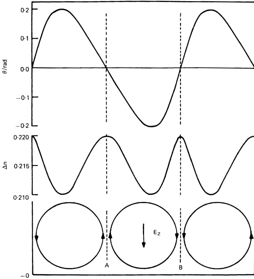
Figure 14. Top: non-sinusoidal director profile obtained from (15). Centre: resulting variation of the effective birefringence \Delta n with X (for n_e = 1.769 , n_o = 1.549 ). Bottom: the disposition of the convective rolls agrees with the observed dust-particle motion, the regions B corresponding to the bright lines of figure 12.
